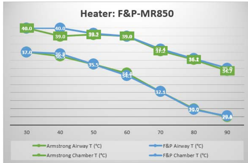
Graph 1. Temperature/Gas Flow variation with Heater F&P-MR850
