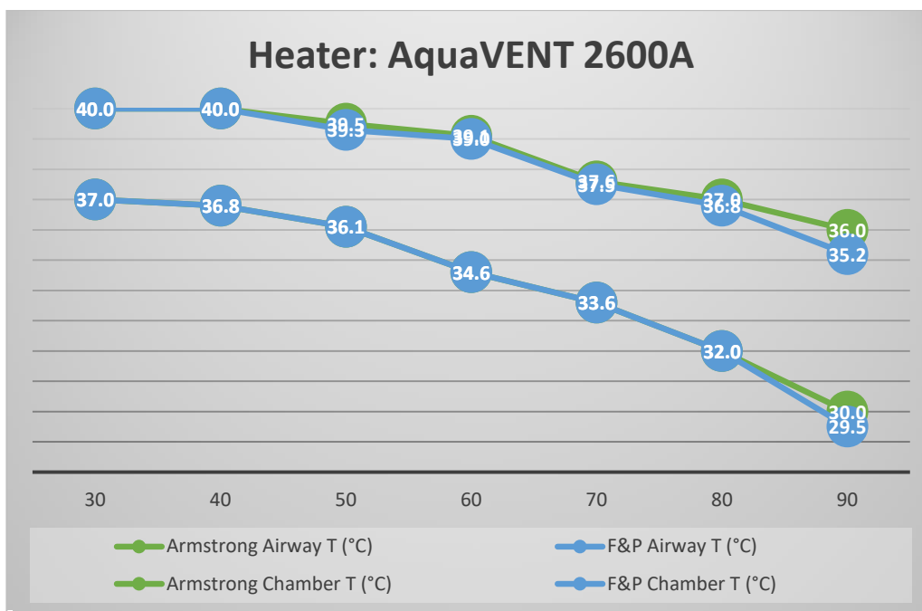
Graph 2. Temperature/Gas Flow variation with Heater AquaVENT 2600A
